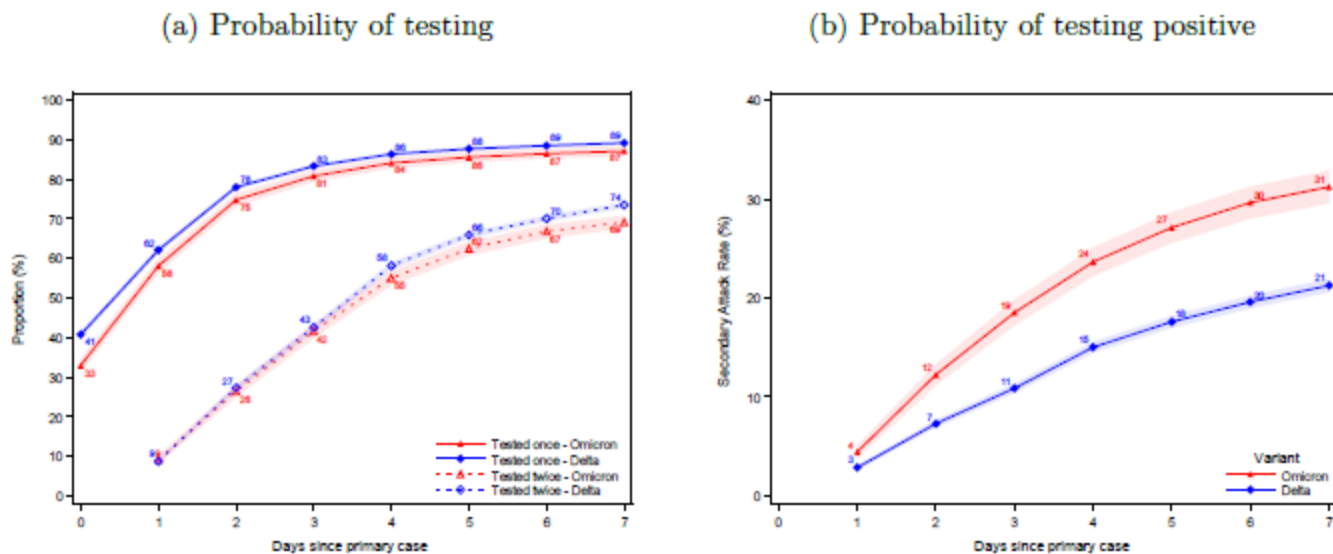
Figure 1: Probability of being tested and testing positive
